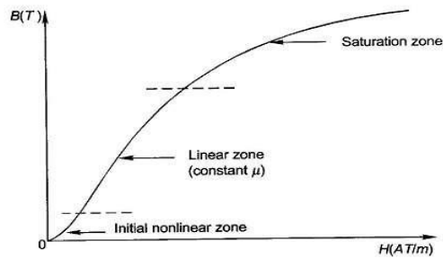
Fig. 2.3 Typical normal magnetization curve of ferromagnetic material
